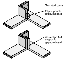
Two-stud Corner
